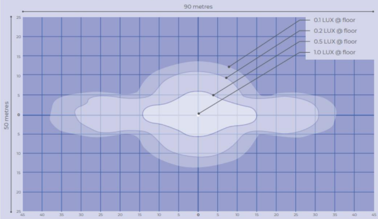
CLIFEM-PRO-SM-WP-WL (C-Plane 2degree) EM550mA Isolux Pattern – 10m Mounting Height
