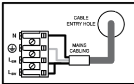
Figure A Permanently on, 24hr operation. The switched active (L sw ) and un-switched active (L em ) connections are bridged ensuring the battery charger and general lighting LED driver is permanently energised.
