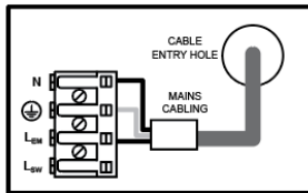
Figure C Non-maintained operation. The switched active (L sw ) is not connected and the general lighting LED driver will be off (permanently). The un-switched active (L em ) supplying battery charger is permanently energised.
