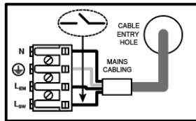
Figure B Switched operation of the general lighting LED driver. The switched active (L sw ) is wired separately via a switch to provide on/off control of the general lighting. The un-switched active (L em ) supplying battery charger is permanently energised.* *The switched and un-switched active should originate from the same circuit breaker or RCD.
