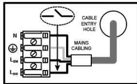
Figure B Switched operation of the general lighting LED driver. The switched active ( L_{sw} ) is wired separately via a switch to provide on/off control of the general lighting. The un-switched active ( L_{em} ) supplying battery charger is permanently energised.* *The switched and un-switched active should originate from the same circuit breaker or RCD.
