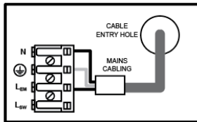
Figure C Non-maintained operation. The switched active ( L_{sw} ) is not connected and the general lighting LED driver will be off (permanently). The un-switched active ( L_{em} ) supplying battery charger is permanently energised.
