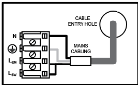
Figure A Permanently on, 24hr operation. The switched active ( L_{sw} ) and un-switched active ( L_{em} ) connections are bridged ensuring the battery charger and general lighting LED driver is permanently energised.
